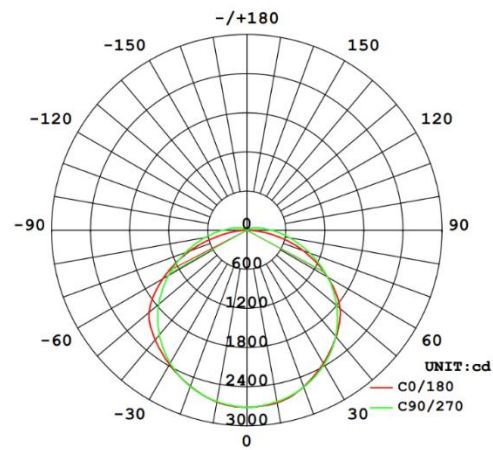
Diagram for RHEE60X6FT-24 in 60W 5000K. Other diagrams available on request
