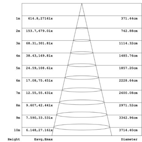
Diagram for RHEE60X6FT-24 in 60W 5000K. Other diagrams available on request
